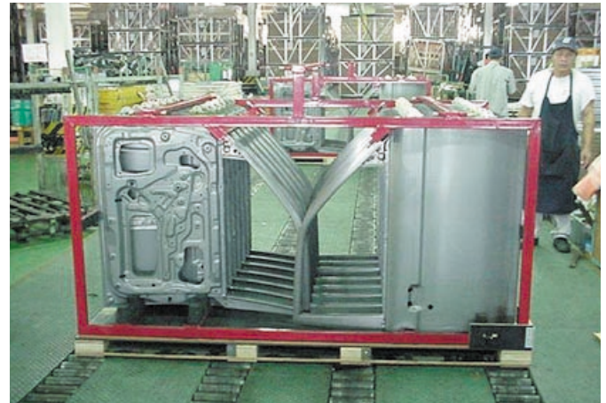
Above: Front doors held in place by tailor made dunnage
