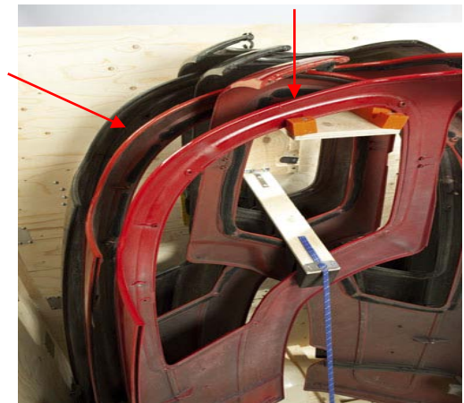
To gain space between the items and avoid scratches during transport, the painted parts are fixed in PUR dunnage
