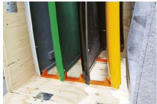
In the bottom the parts are placed in PUR separators to secure their position during transport
