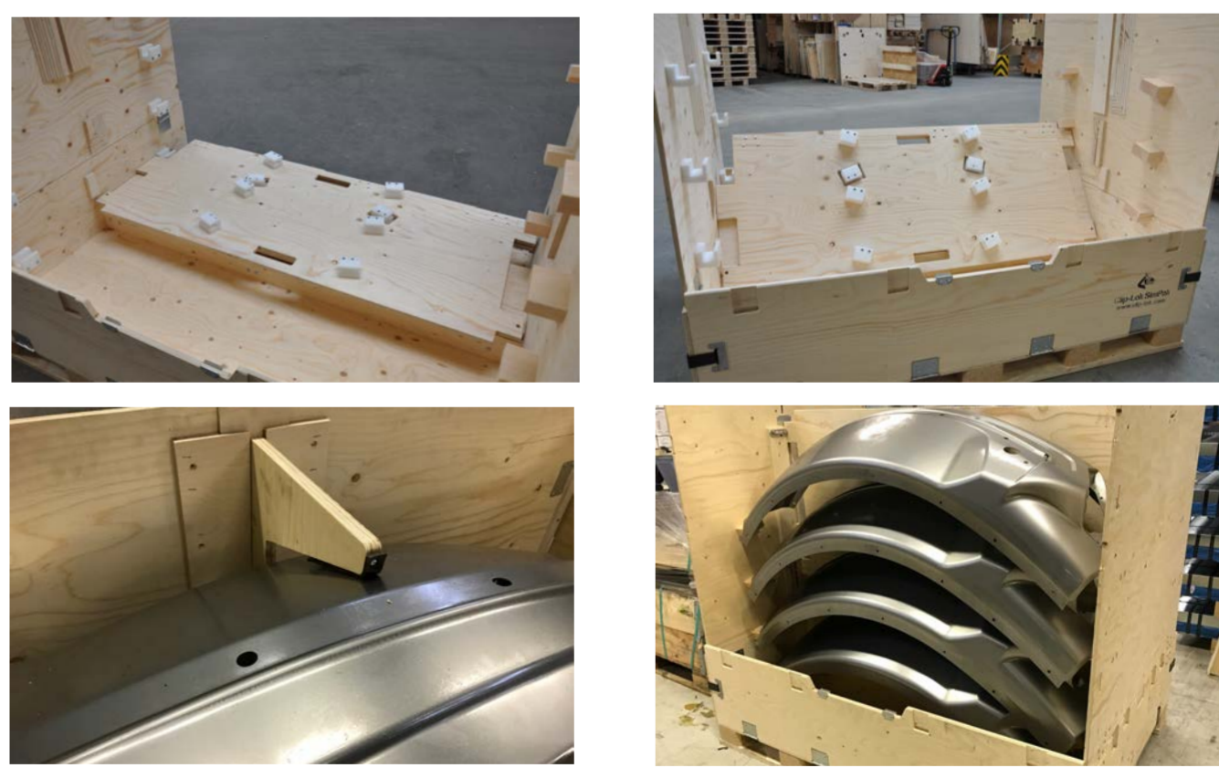
Different phases of the Clip-Lok 2P box assembly. The locking feature on top secures a box of fully loaded fenders during transport.
