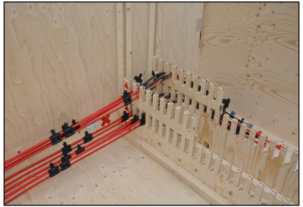
The custom designed plywood dunnage is 35% stronger than the cardboard alternative, providing better support and security to the Busbars during shipping and thus saving costs.
