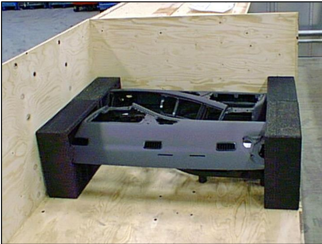
The first two dashboards are packed in place. Each custom designed EPP shell fits both right- and left-side dashboards, so no extra dunnage sets are necessary.
