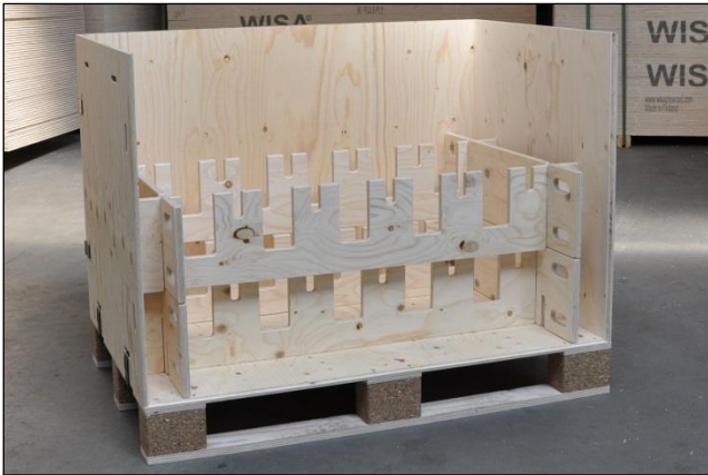
The support racks are built up, as layers of rifles are added. There is no need for extra packaging material.
