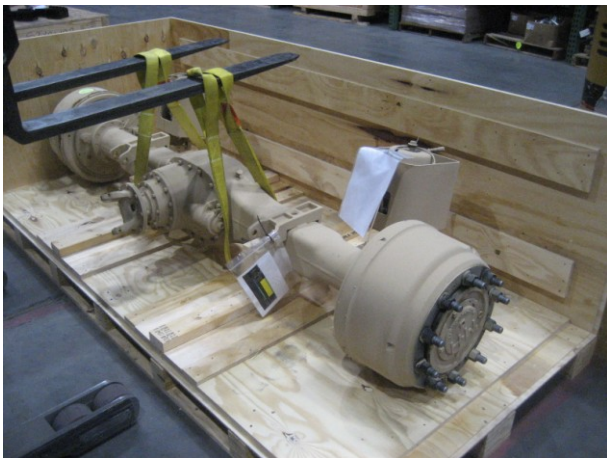
The design of the Clip-Lok box allows easy access when loading the axle with forklift
